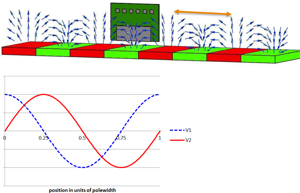
Figure 2: typical application of a PCB mounted KMP sensor moving relative to a magnetic pole and the corresponding output signal voltage depending on sensor position
