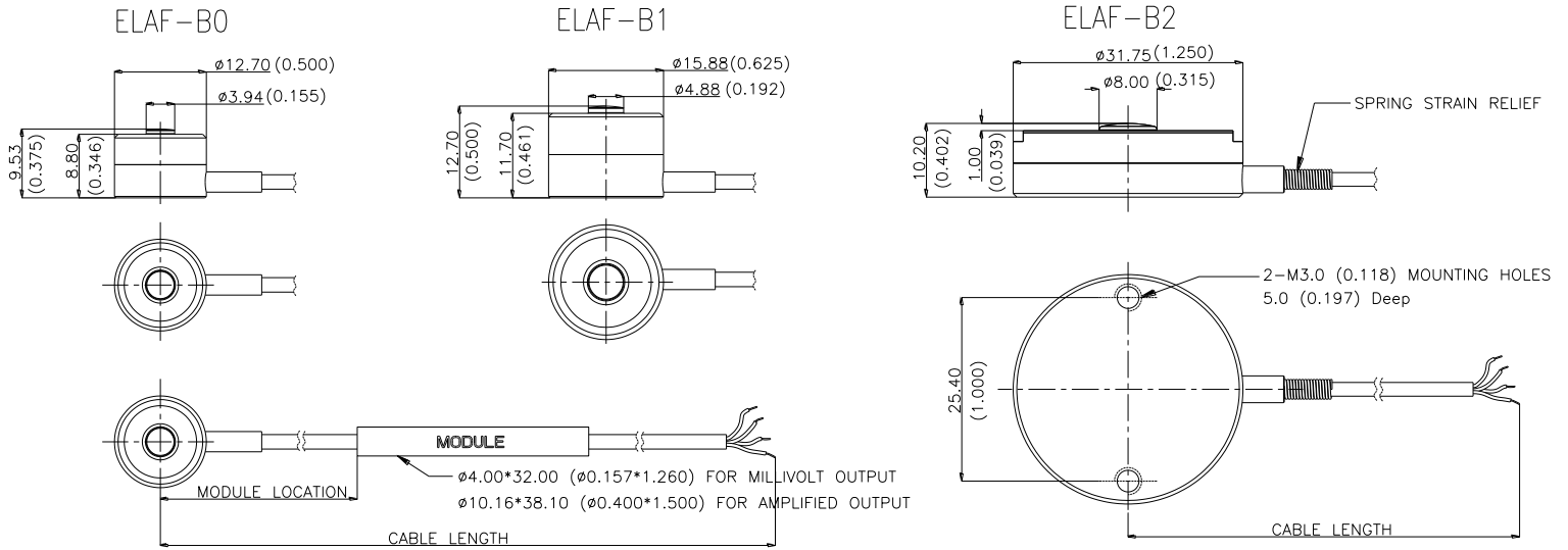
ELAF-B0 FORCE
