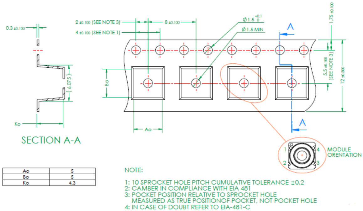
Figure 16: Tape and Reel
