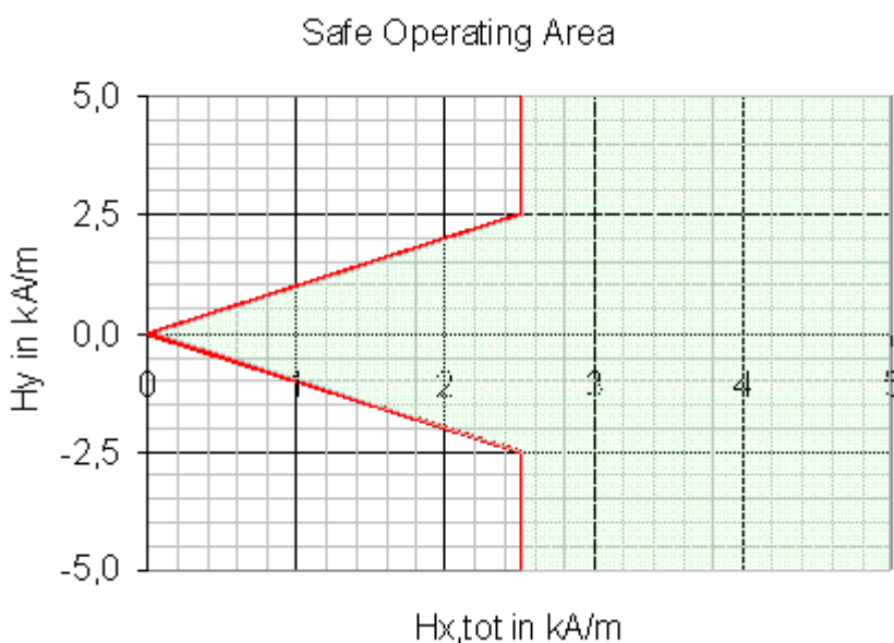
Figure 2: Safe operating area
