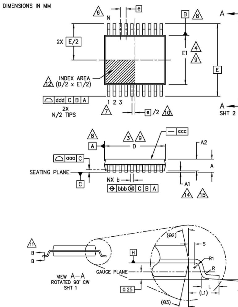
Figure 8: Package drawing
